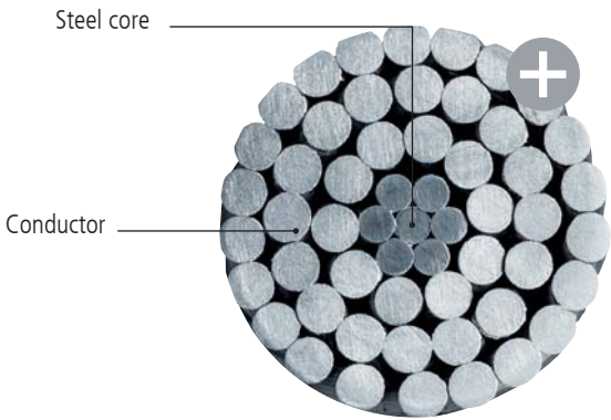
The outer area of these conductor cables consists of light, highly conductive aluminium wires, while the core is made of specially stretch-resistant, galvanised steel wires
